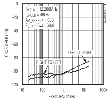
CROSSTALK vs. FREQUENCY (DAC TO SPEAKER)
