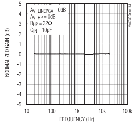
GAIN vs. FREQUENCY (LINE TO HEADPHONE)
