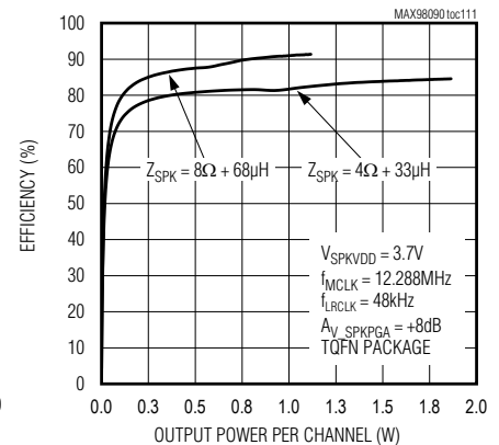
EFFICIENCY vs. OUTPUT POWER (DAC TO SPEAKER)
