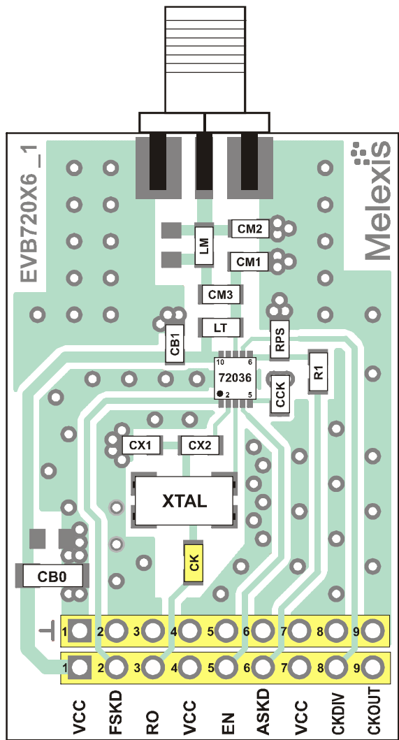
Board size is 27 mm x 42 mm
