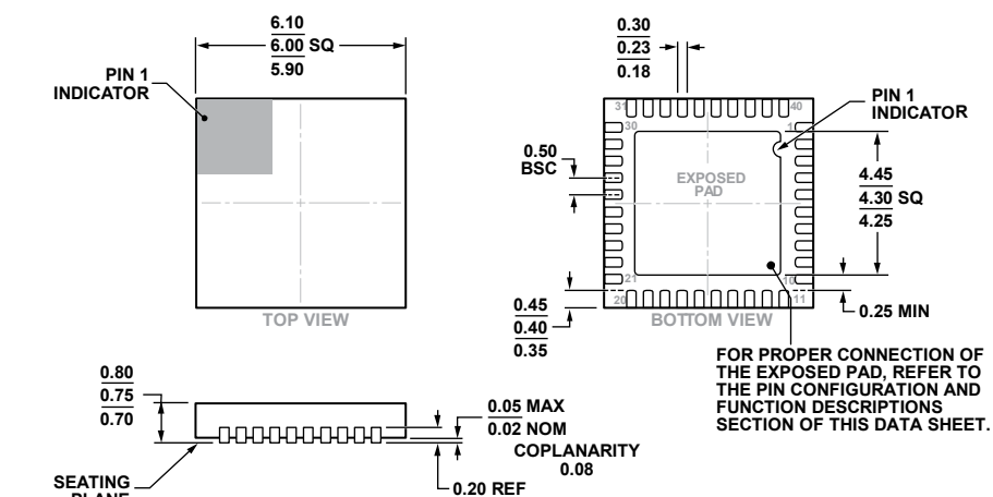
Figure 52. 40-Lead Lead Frame Chip Scale Package [LFCSP] 6 mm × 6 mm Body and 0.75 mm Package Height (CP-40-10)
