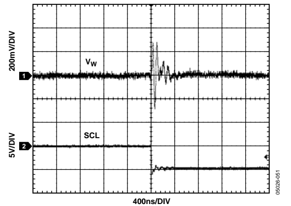
Figure 29. Digital Feedthrough
