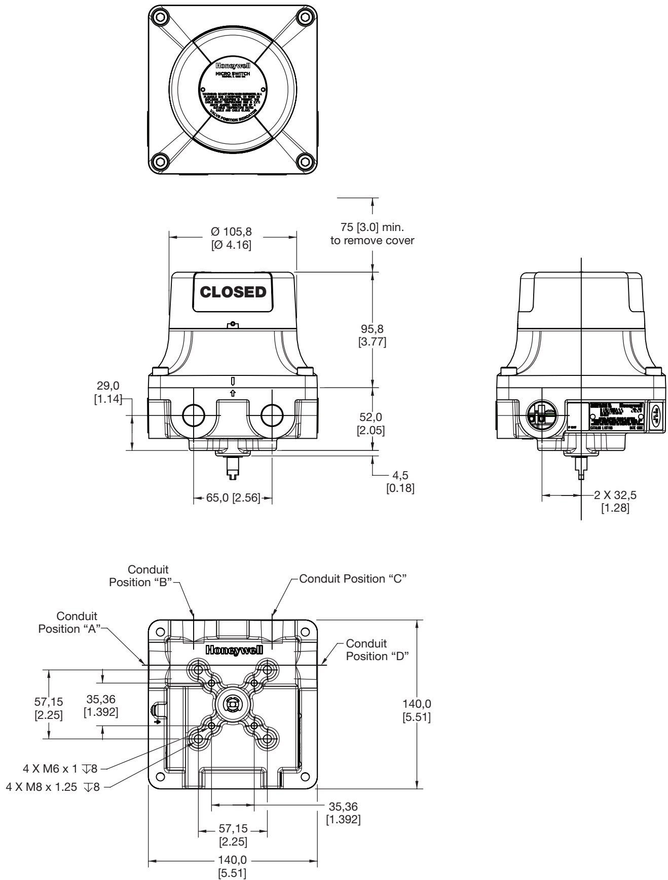
FIGURE 2. MOUNTING DIMENSIONS
