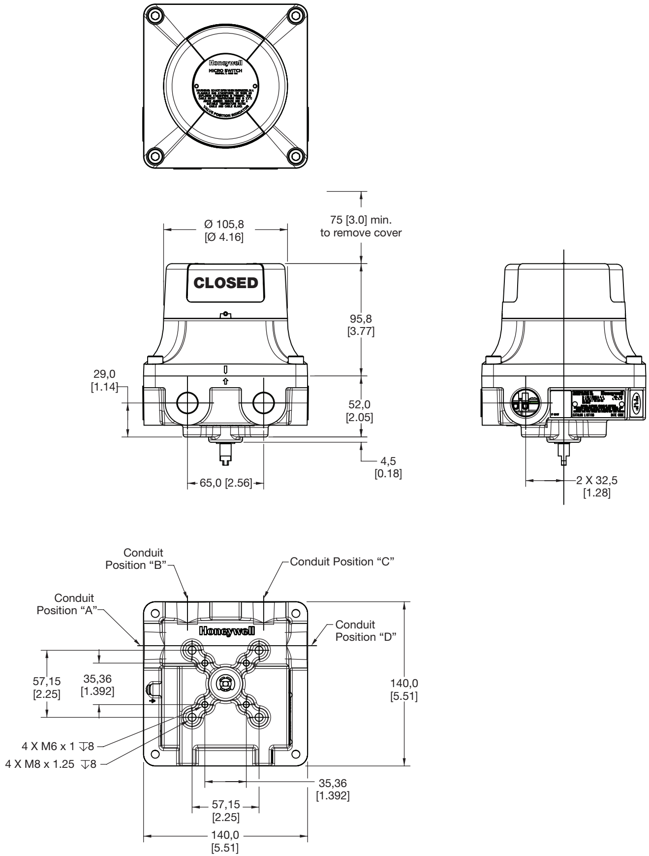
FIGURE 2. MOUNTING DIMENSIONS
