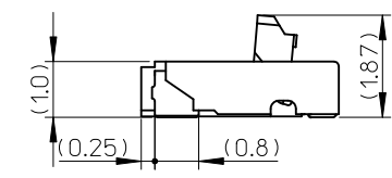
SECTION Y-Y
