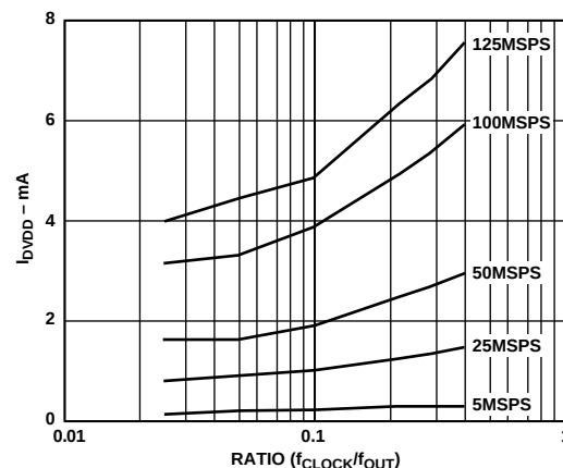
Figure 27. I_{DVDD} vs. Ratio @ DVDD = 3\text{ V}
