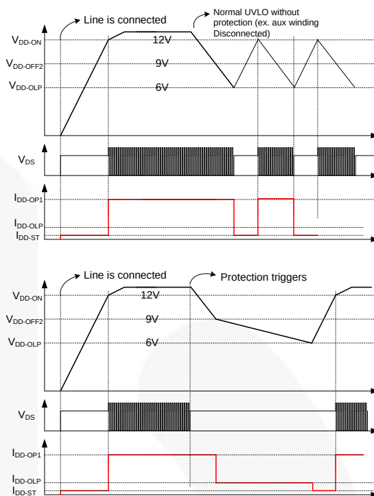
Figure 26. Two-Level UVLO
