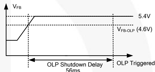
Figure 25. OLP Operation
