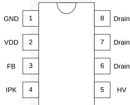
Figure 4. Pin Assignment
