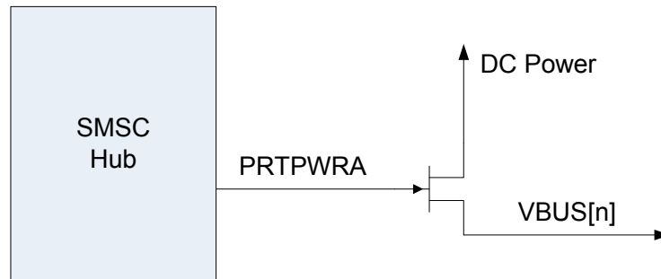
Figure 8.1 Battery Charging External Power Supply
