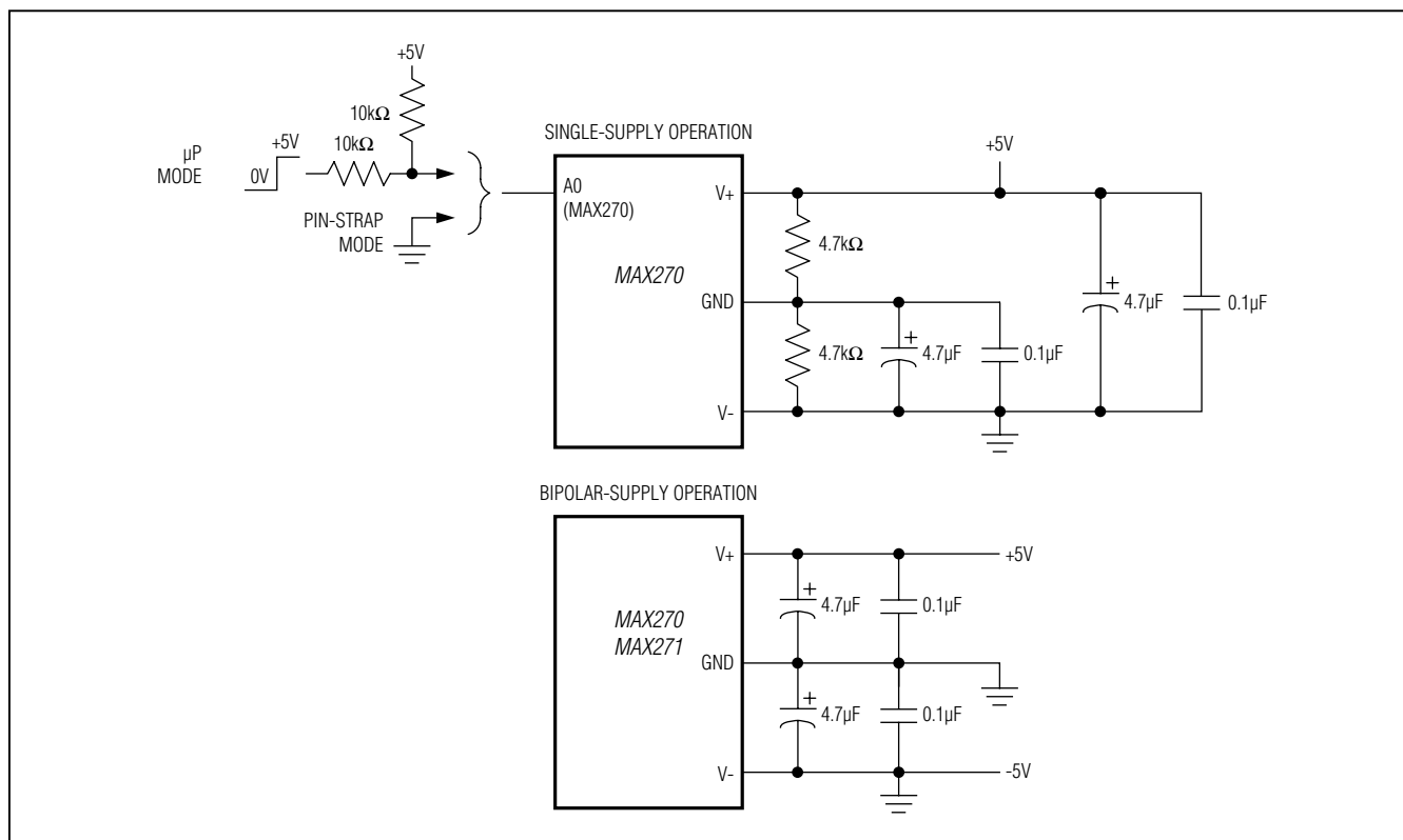
Figure 4. Power-Supply Configurations
