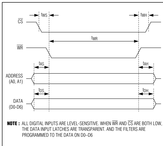
Figure 2. MAX270/MAX271 Digital Timing Diagram
