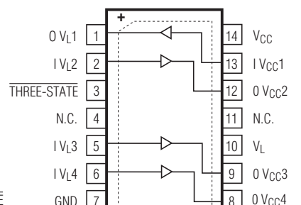
TDFN-14 (3mm x 3mm) TOP VIEW
