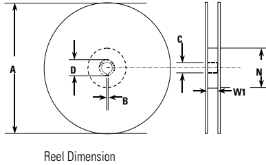
Reel Dimension
