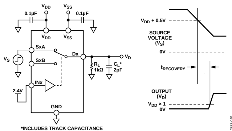
Figure 40. Overvoltage Recovery Time, t_{\text{RECOVERY}}
