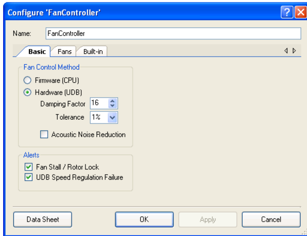
Figure 4-19 Example2 Fan Controller Customizer – Basic Tab
