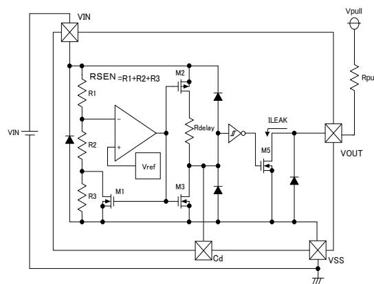
Note: R_{OFF} = V_{OUT} / I_{LEAK} Figure 4: Circuit example of XC6109N Series
