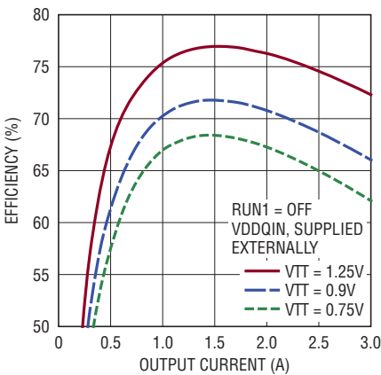
Figure 3. VTT 12VIN Efficiency
