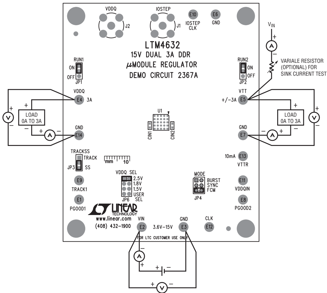
Figure 1. Test Setup
