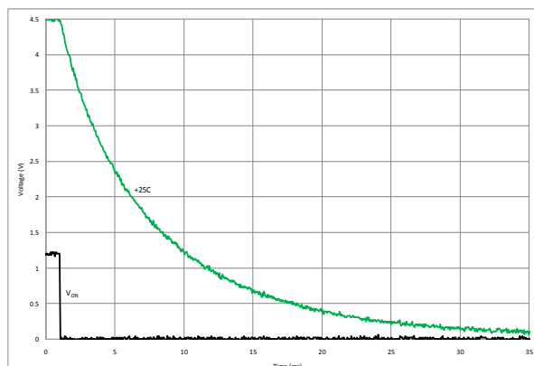
Figure 29. Turn-Off Response ( V_{IN}=4.5 V, C_{IN}=10 \mu F, C_L=100 \mu F, without External R_L )
