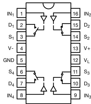
DG413LE Dual-In-Line, TSSOP and SOIC
