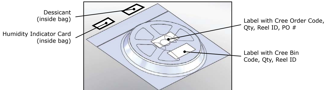
Packaged Reel
