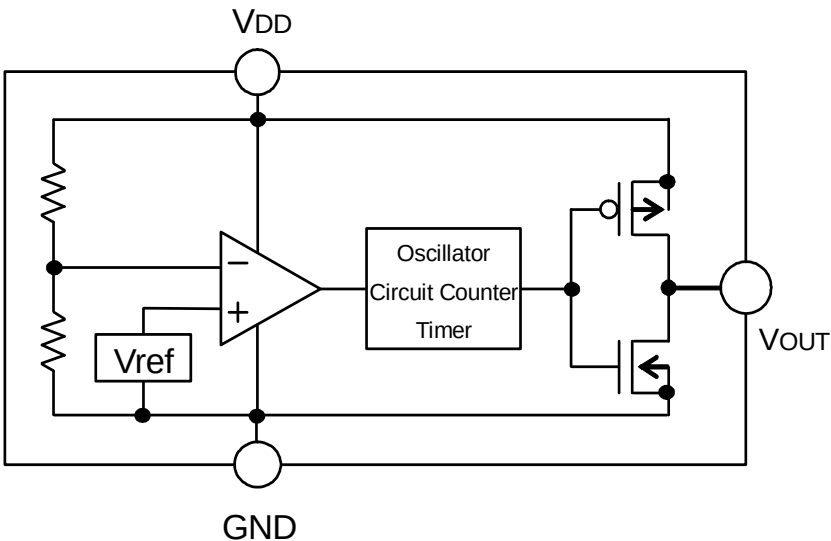
Fig.2 BU46xxxxx Series
