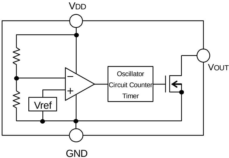
Fig.1 BU45xxxxx Series
