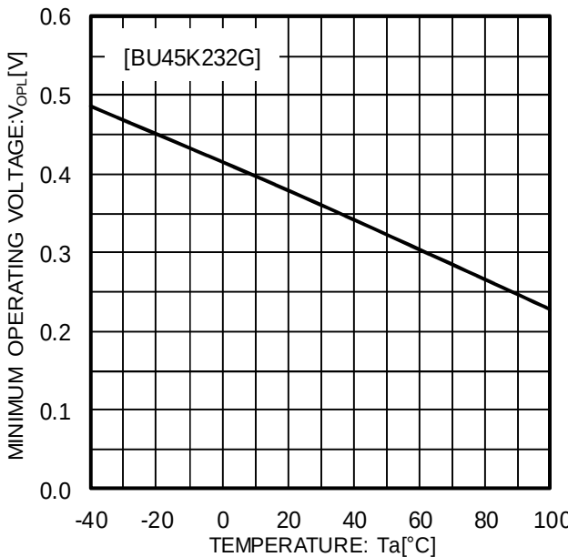
Fig.10 Operating Limit Voltage
