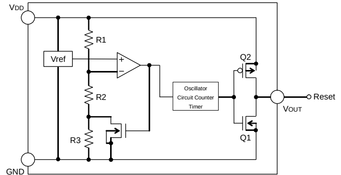
Fig.14 (BU46xxxxx Type Internal Block Diagram)
