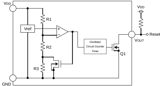
Fig.13 (BU45xxxxx Type Internal Block Diagram)
