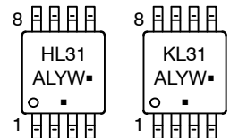
TSSOP-8 DT SUFFIX CASE 948R
