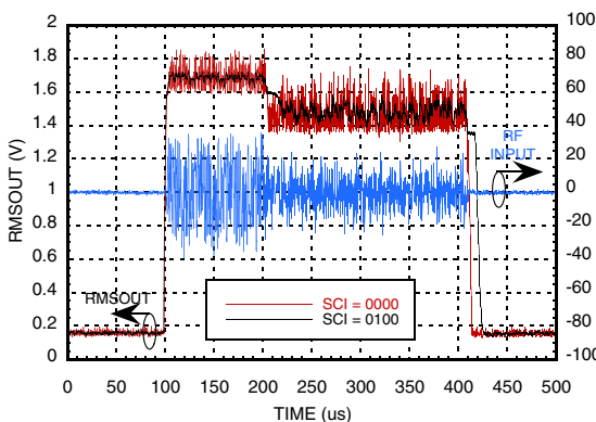
Residual Ripple for 900 MHz WiMAX @ SCI=0100
