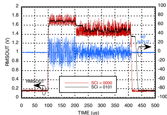
Residual Ripple for 900 MHz WiMAX @ SCI=0101
