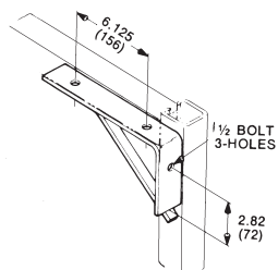
Angle Bracket
