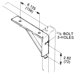
Angle Bracket
