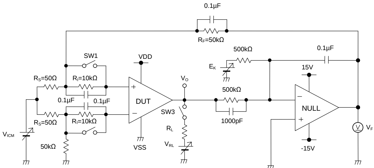
Figure 74. Test Circuit 1
