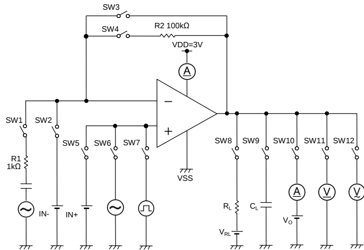
Figure 75. Test Circuit2
