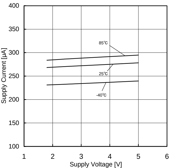
Figure 53. Supply Current vs Supply Voltage
