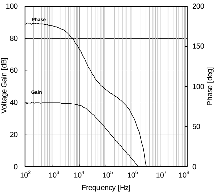
Figure 48. Voltage Gain · Phase vs Frequency
