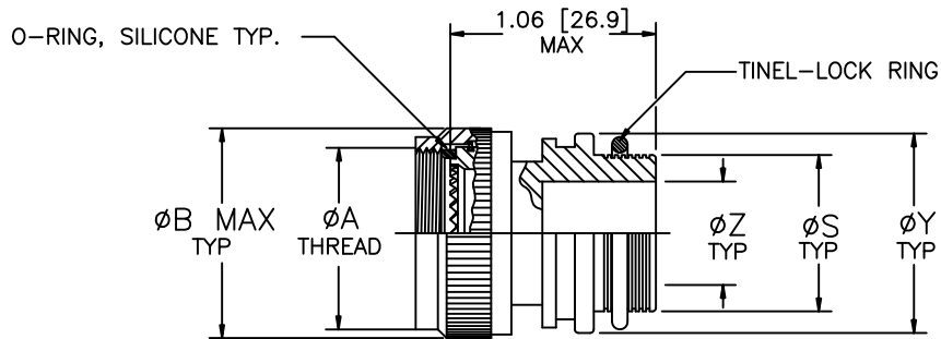
FIGURE 1 STRAIGHT ADAPTER
