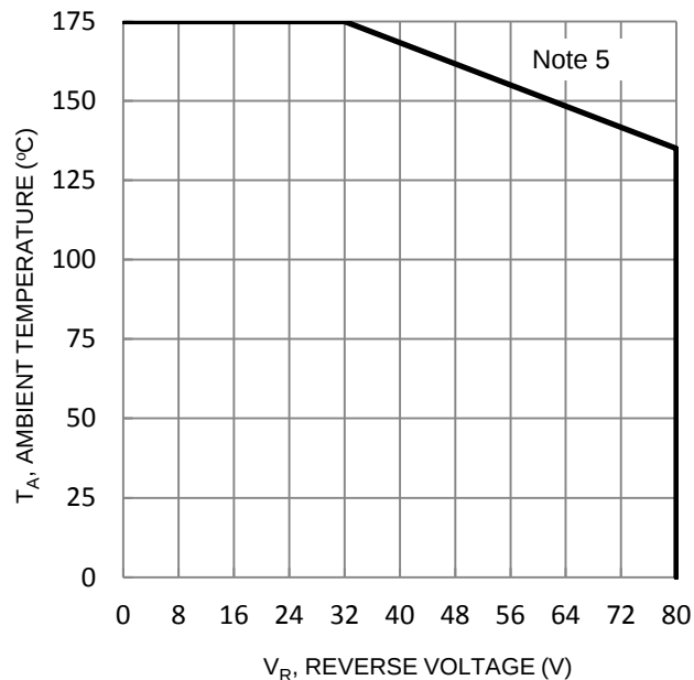
Fig.4 Operating Temperature Derating
