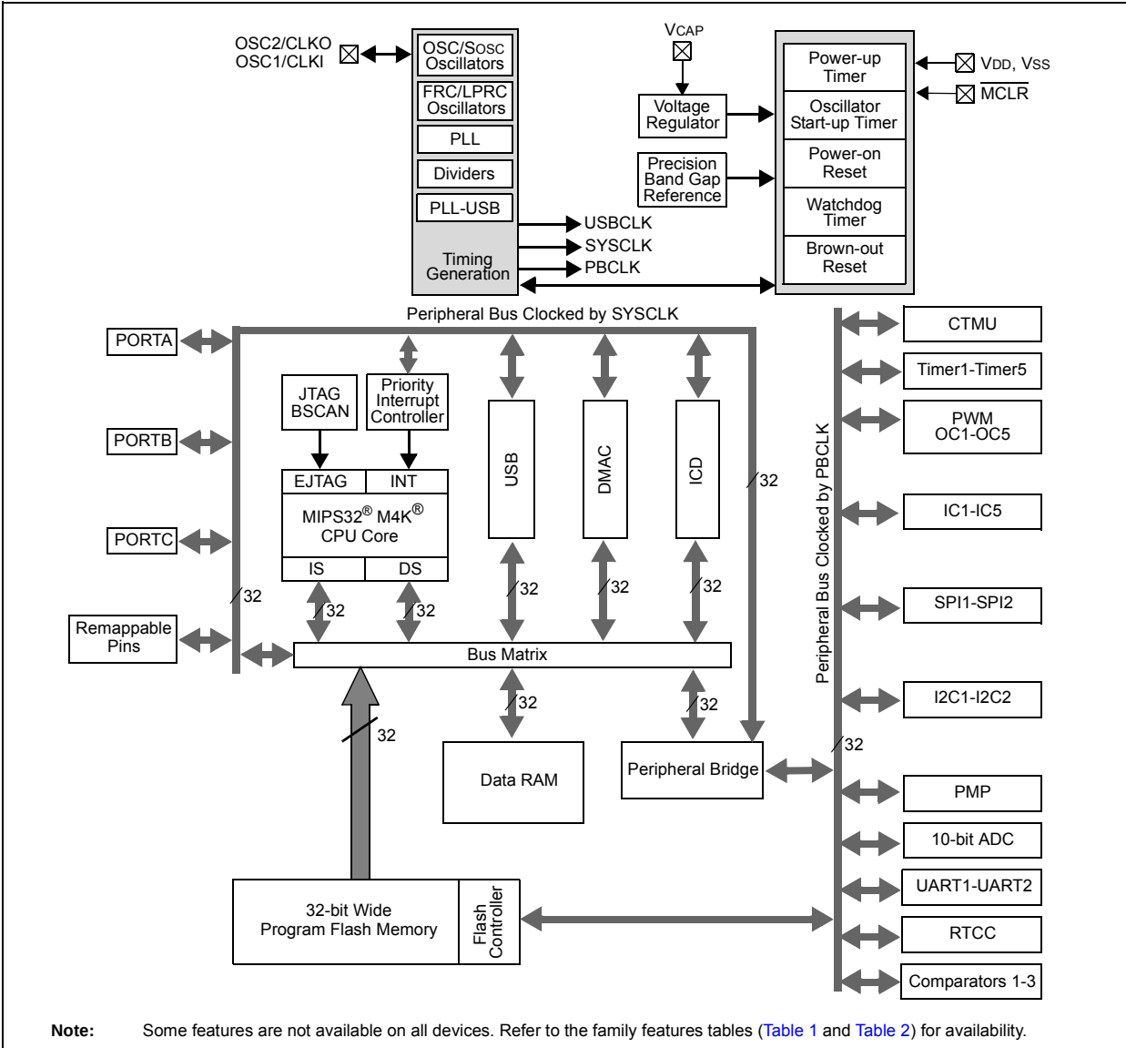
FIGURE 1-1: BLOCK DIAGRAM
