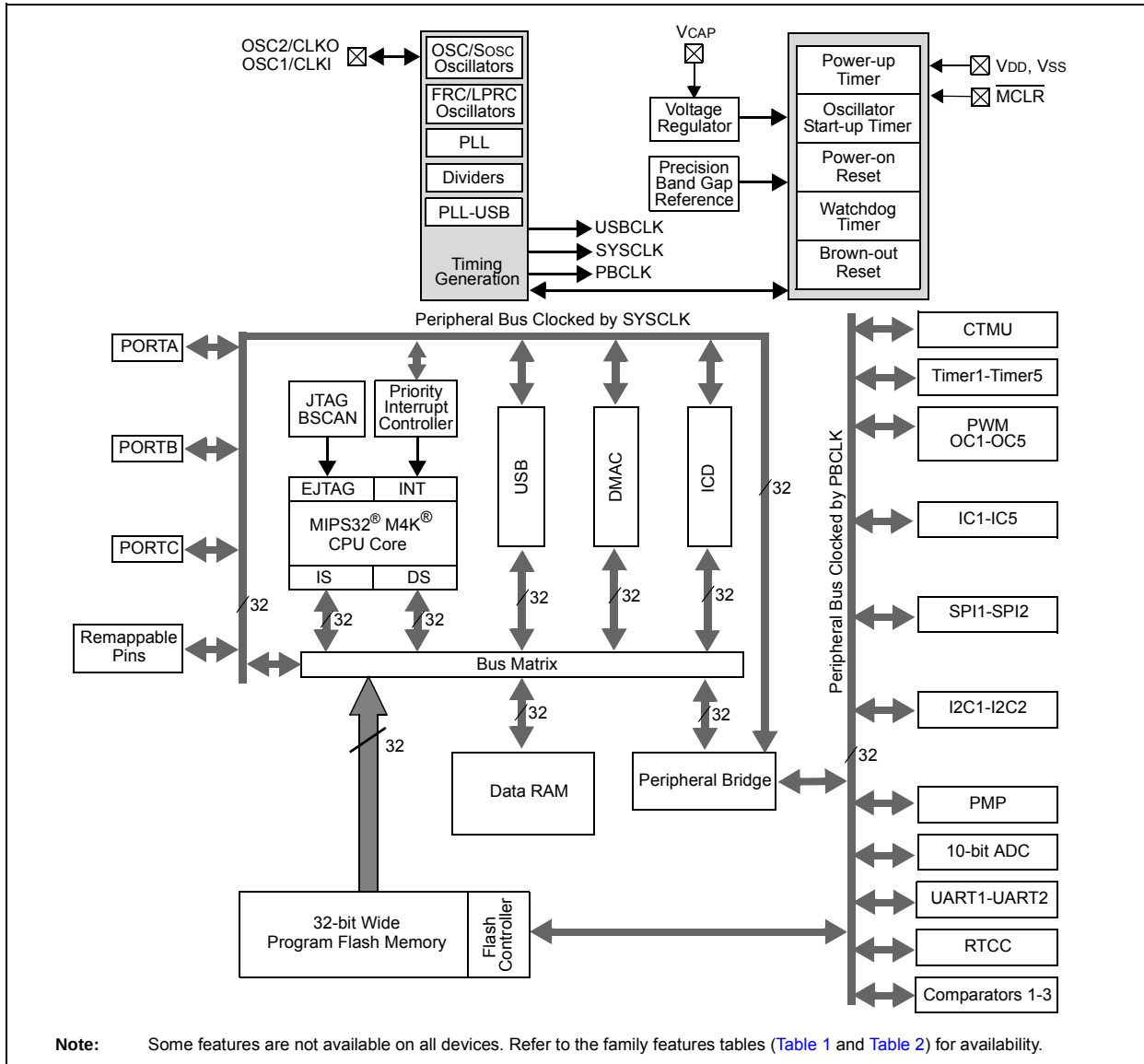
FIGURE 1-1: BLOCK DIAGRAM
