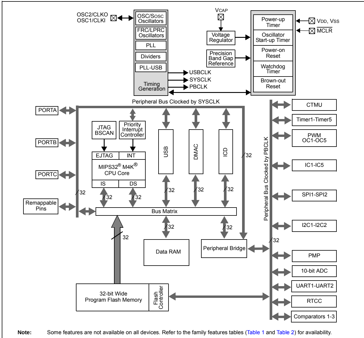
FIGURE 1-1: BLOCK DIAGRAM
