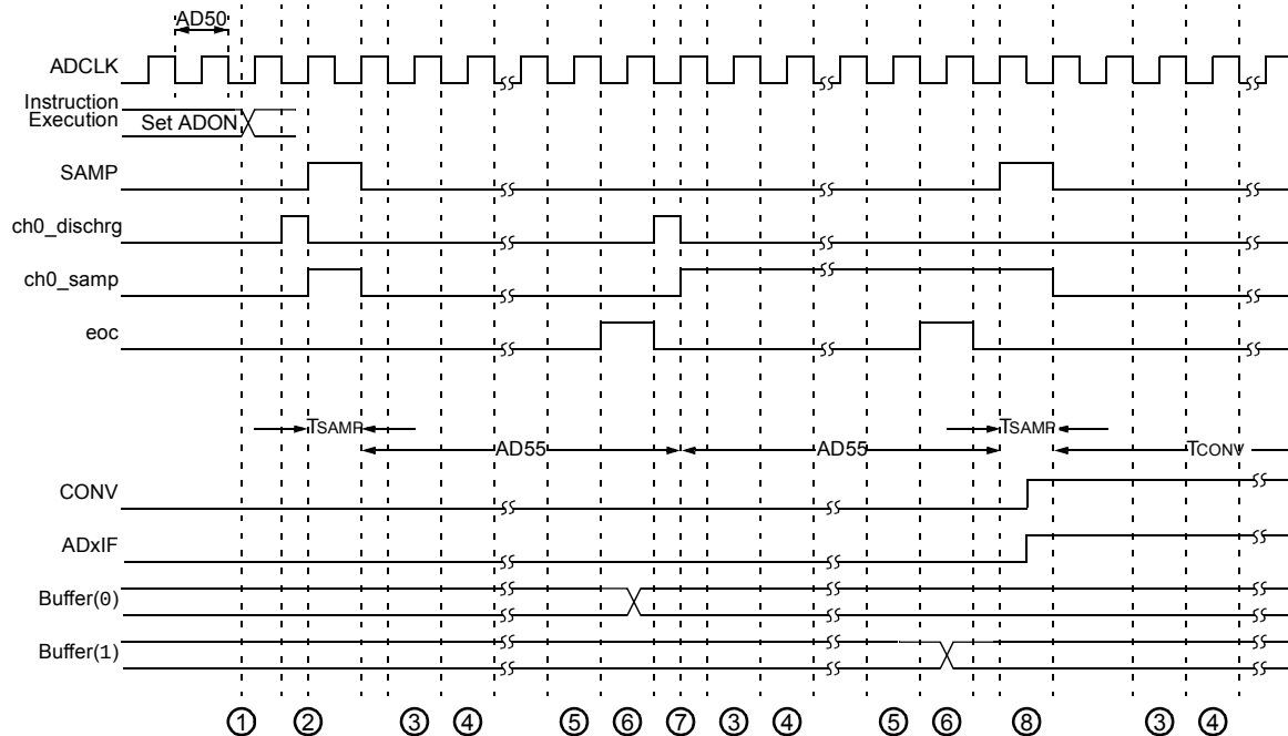
FIGURE 30-19: ANALOG-TO-DIGITAL CONVERSION (10-BIT MODE) TIMING CHARACTERISTICS (ASAM = 1, SSRC<2:0> = 111, SAMC<4:0> = 00001)
