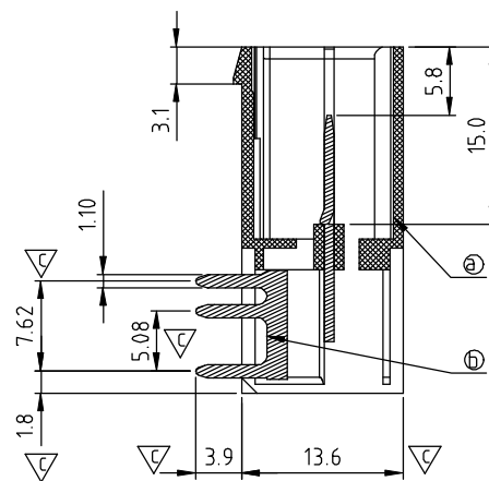
SECTION P-P
