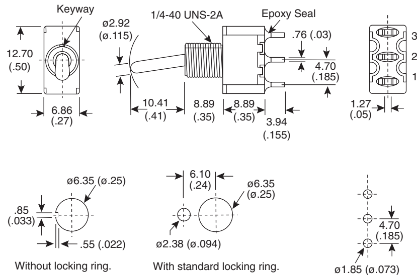
PANEL MOUNTING
