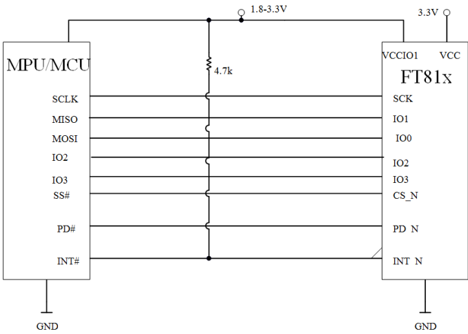
Figure 9: Quad channel SPI Interface connection
