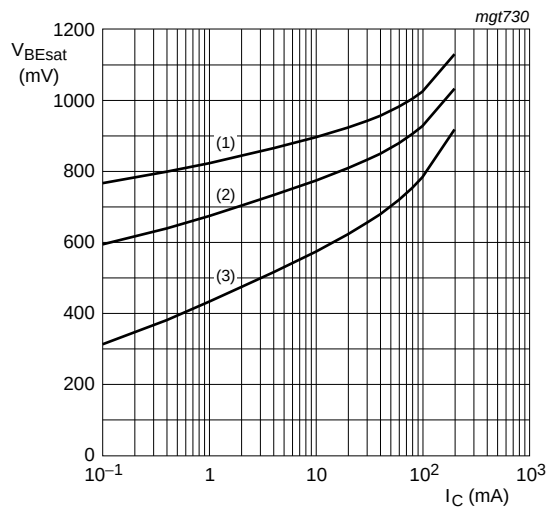
Fig 8. BC847BMB: Base-emitter voltage as a function of collector current; typical values
