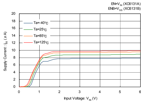
XC6131 ( V_{DF(T)}=3.0V )
