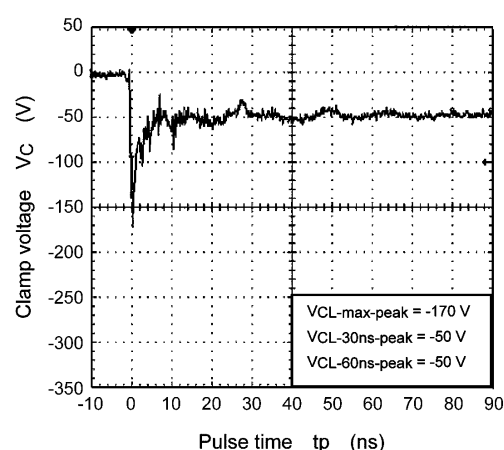
Fig. 10.2 -8 kV (IEC61000-4-2)
