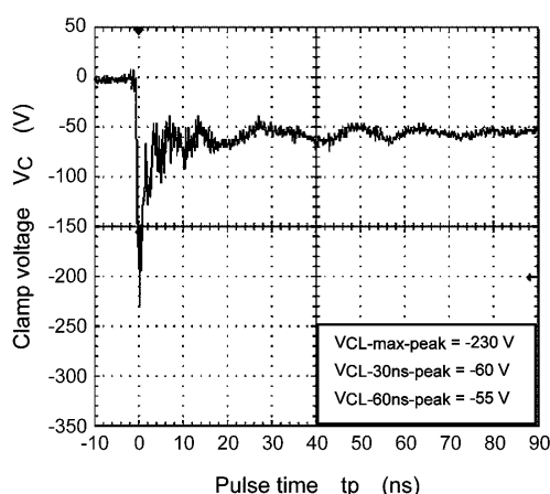
Fig. 11.4 -15 kV (ISO10605)
