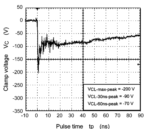
Fig. 10.4 -15 kV (IEC61000-4-2)
