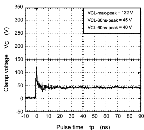
Fig. 11.1 +8 kV (ISO10605)
