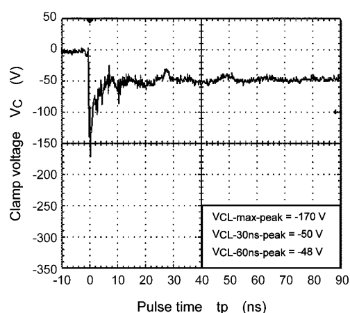
Fig. 11.2 -8 kV (ISO10605)
