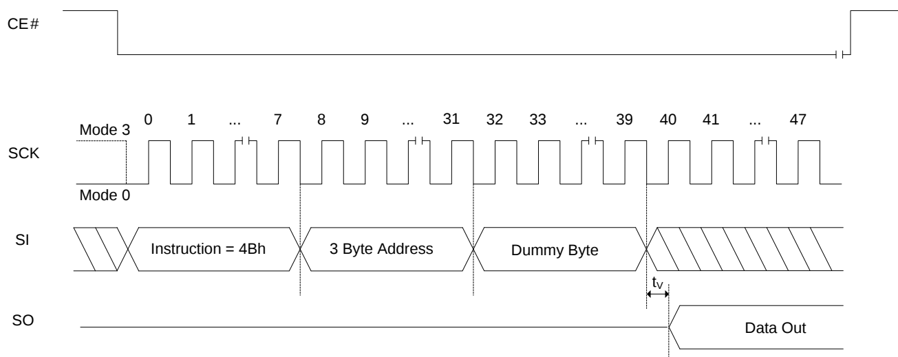
Figure 8.25 RDUID Operation
