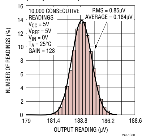
Noise Histogram (2x Speed Mode)
