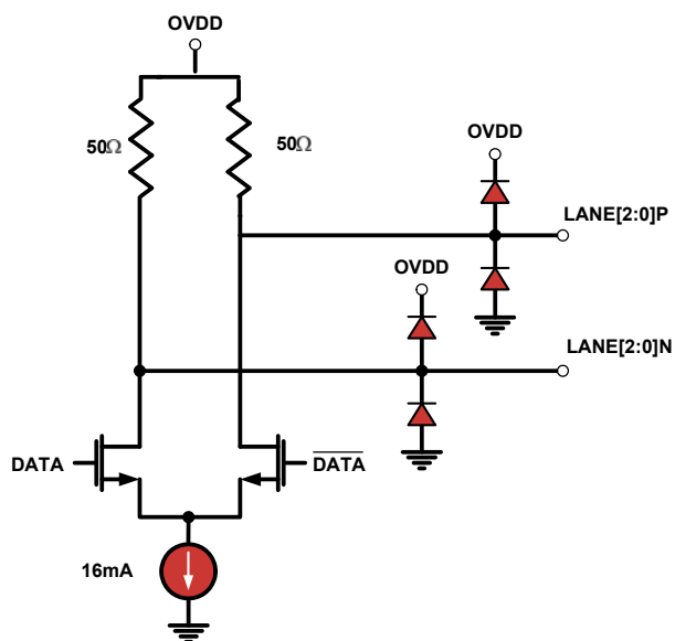
FIGURE 62. CML OUTPUTS
