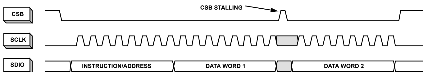
FIGURE 56. 2-BYTE TRANSFER
