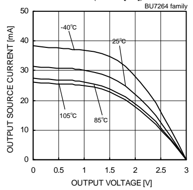
Fig.55 Output Source Current – Output Voltage (VDD=3[V])
