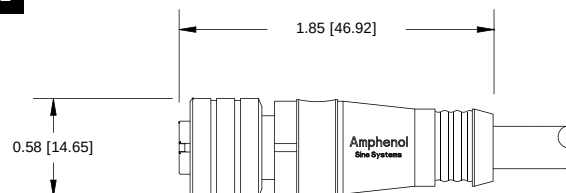
DIMENSIONS - Female Straight
