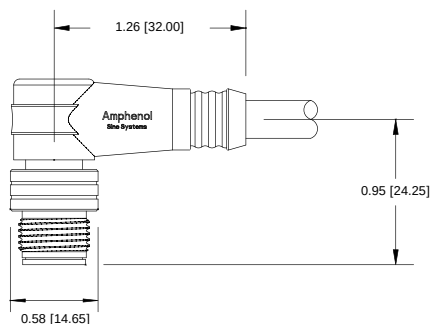
DIMENSIONS - Male 90°
