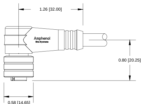
DIMENSIONS - Female 90°
