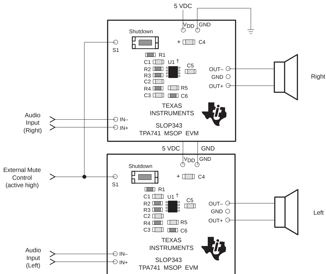
Figure 2–3. TPA741 MSOP EVM Connected for Stereo BTL Output
