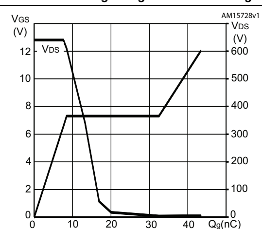
Figure 13. Gate charge vs gate-source voltage
