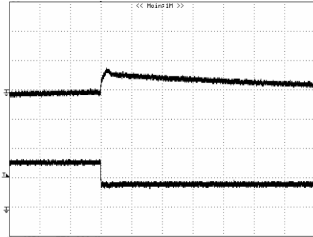
Figure 8: Output voltage response to step-change in load current (50%-25% of I_o , max; di/dt = 0.1A/\mu s ). Load cap: 47 \mu F aluminum capacitor and 1 \mu F ceramic capacitor. TOP Trace: V_{out} (1V/div), Bottom Trace: I_{out} (1A/div), Scope measurement should be made using a BNC cable (length shorter than 20 inches). Position the load between 51 mm to 76 mm (2 inches to 3 inches) from the module.
